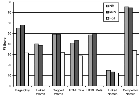
(a) Hoovers-28, micro-avg F_1
